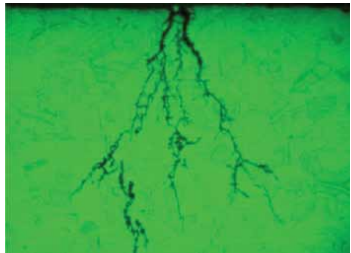
Figure 13: This magnified cross-section of a sample from the roof deck illustrates the extensive SCC that occurred. Photo courtesy of TMR Consulting
