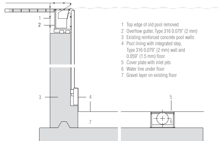
Figure 9: The relining process is shown in this illustration. Courtesy of EuroInox.
